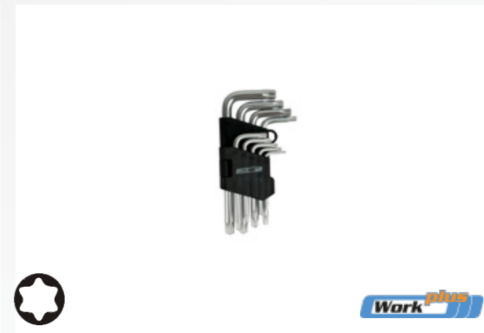
Star hex key set 9pcs Technical: 9 x T10-15-20-25-27-30-40-45-50 x 117 mm Art. nr.: 32108 Packaging: 48 6 Barcode: 8714892321083
